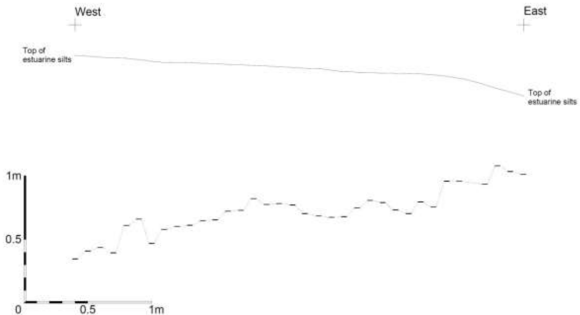
Figure 8: Profile 3 along the width of Wreck 3 (southern profile), with readings taken every 10cm. Depths shown are to the top of solid timbers
