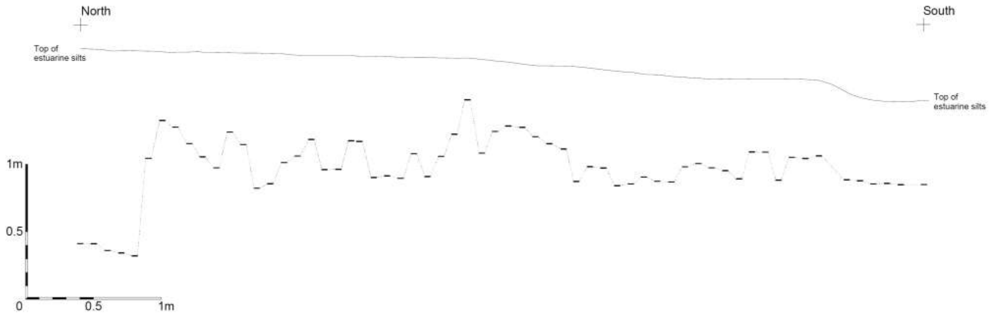
Figure 6: Profile 1 along the centre line of Wreck 3, with readings taken every 10cm. depths shown are to the top of solid timbers
